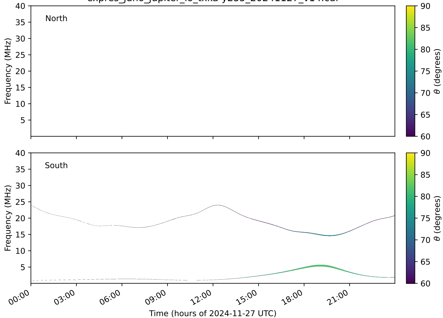
expres_juno_jupiter_io_txka-y235_20241127_v14.cdf
