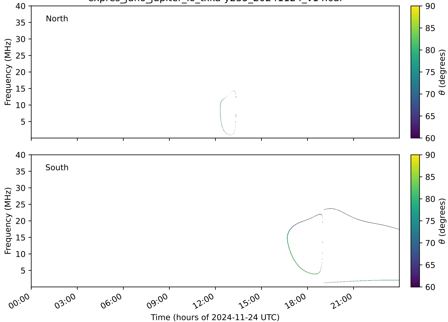
expres_juno_jupiter_io_txka-y235_20241124_v14.cdf
