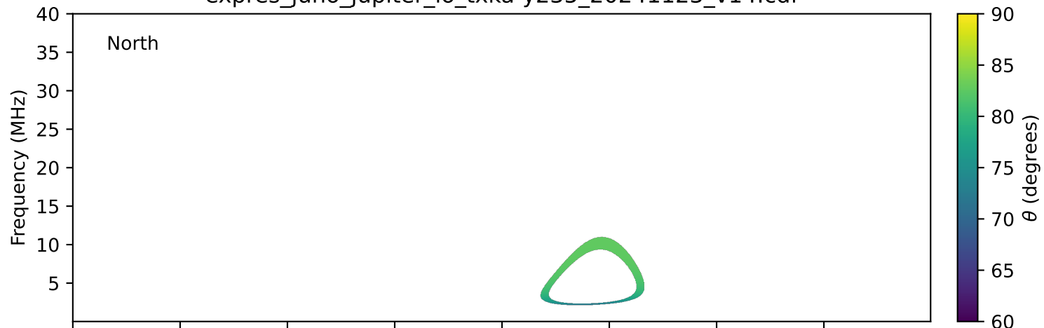
expres_juno_jupiter_io_txka-y235_20241123_v14.cdf
