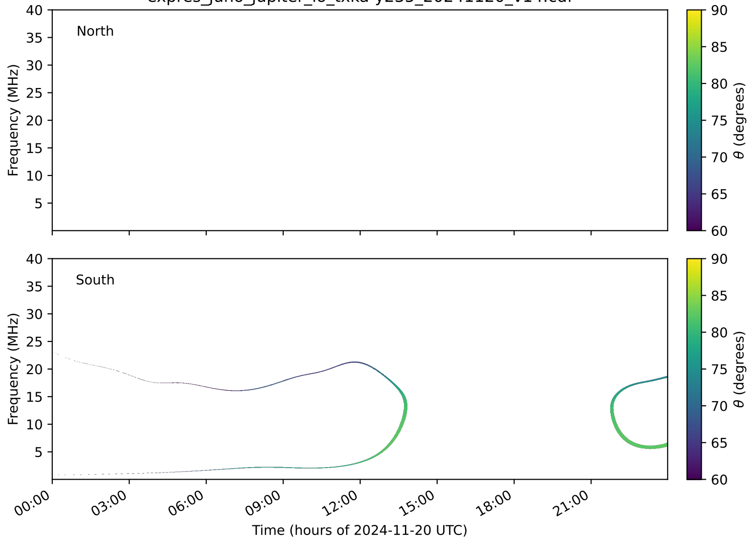
expres_juno_jupiter_io_txka-y235_20241120_v14.cdf
