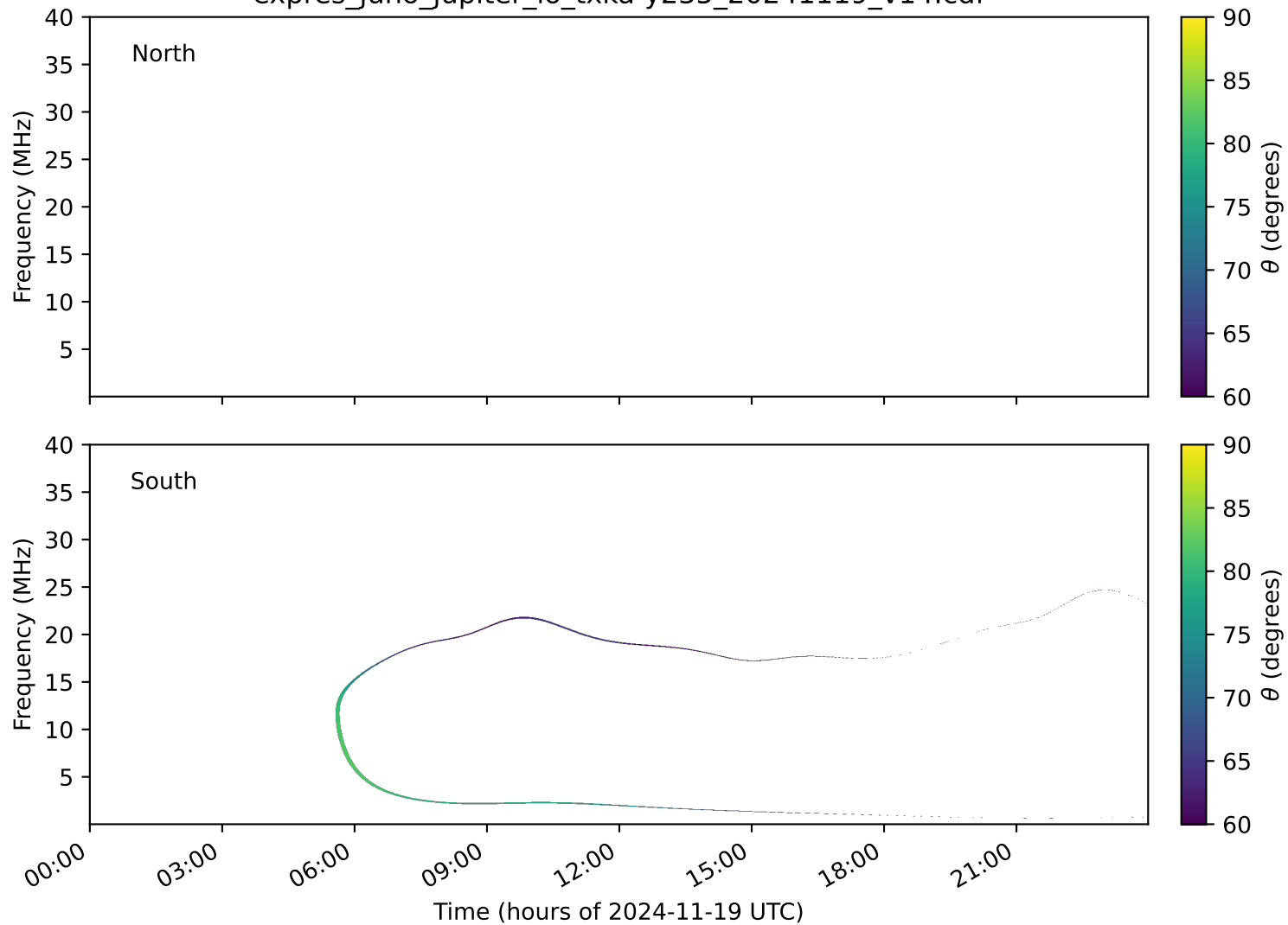
expres_juno_jupiter_io_txka-y235_20241119_v14.cdf
