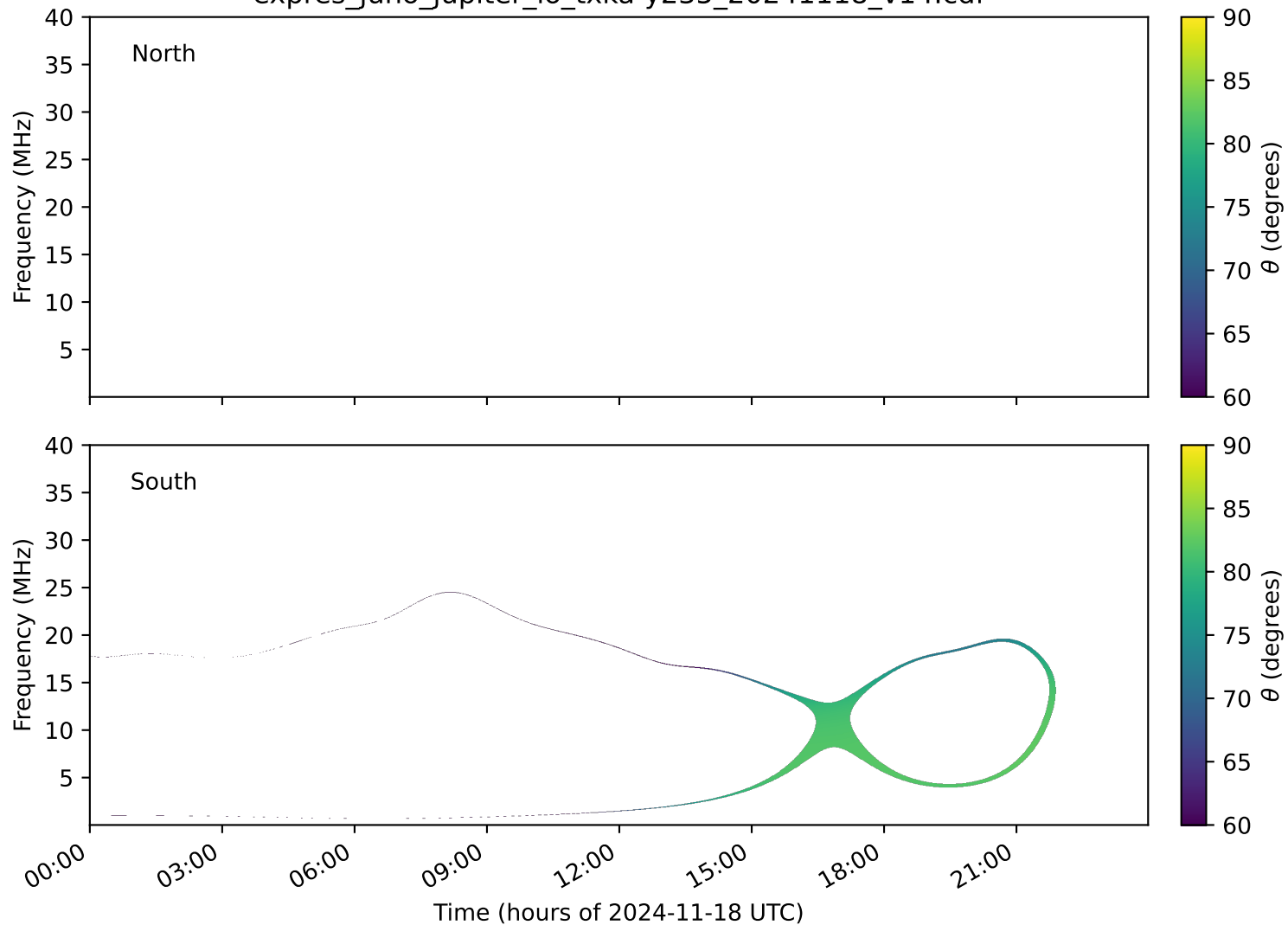
expres_juno_jupiter_io_txka-y235_20241118_v14.cdf
