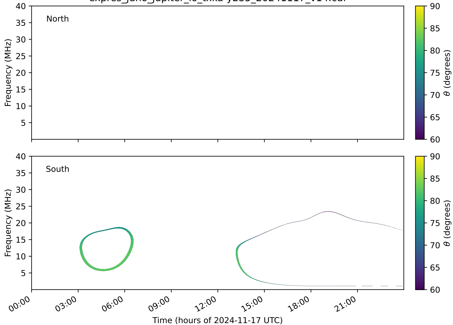
expres_juno_jupiter_io_txka-y235_20241117_v14.cdf
