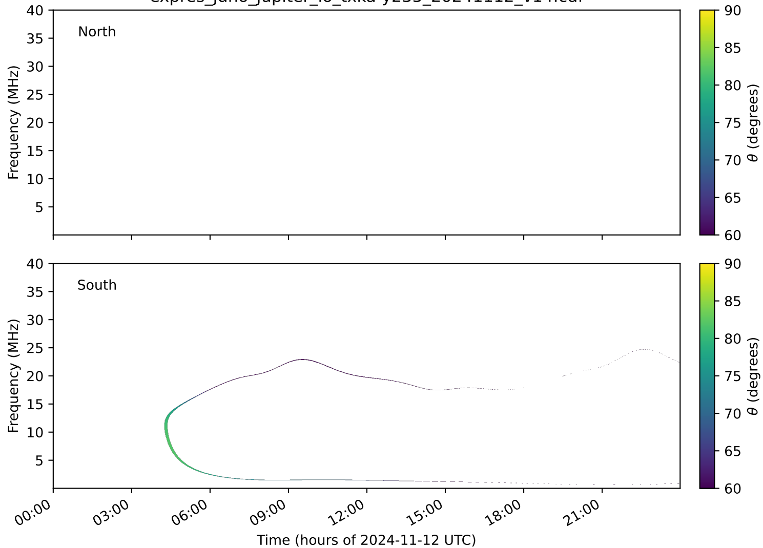
expres_juno_jupiter_io_txka-y235_20241112_v14.cdf
