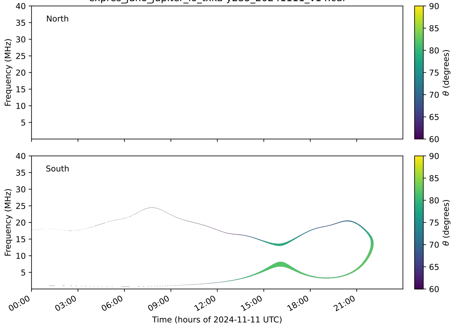
expres_juno_jupiter_io_txka-y235_20241111_v14.cdf
