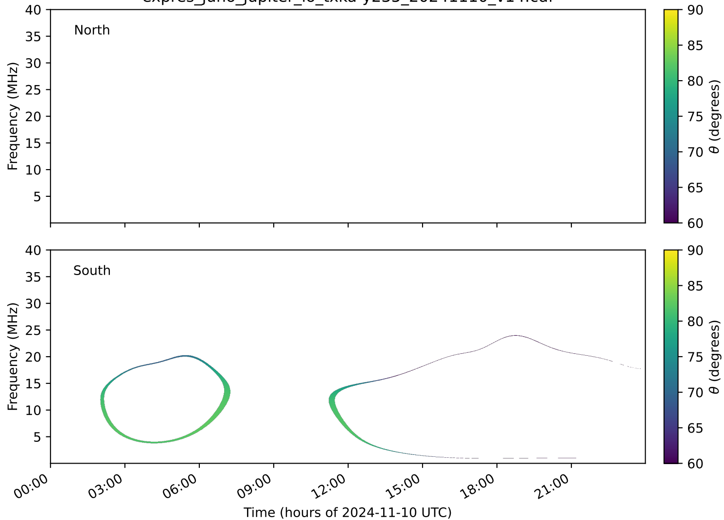
expres_juno_jupiter_io_txka-y235_20241110_v14.cdf
