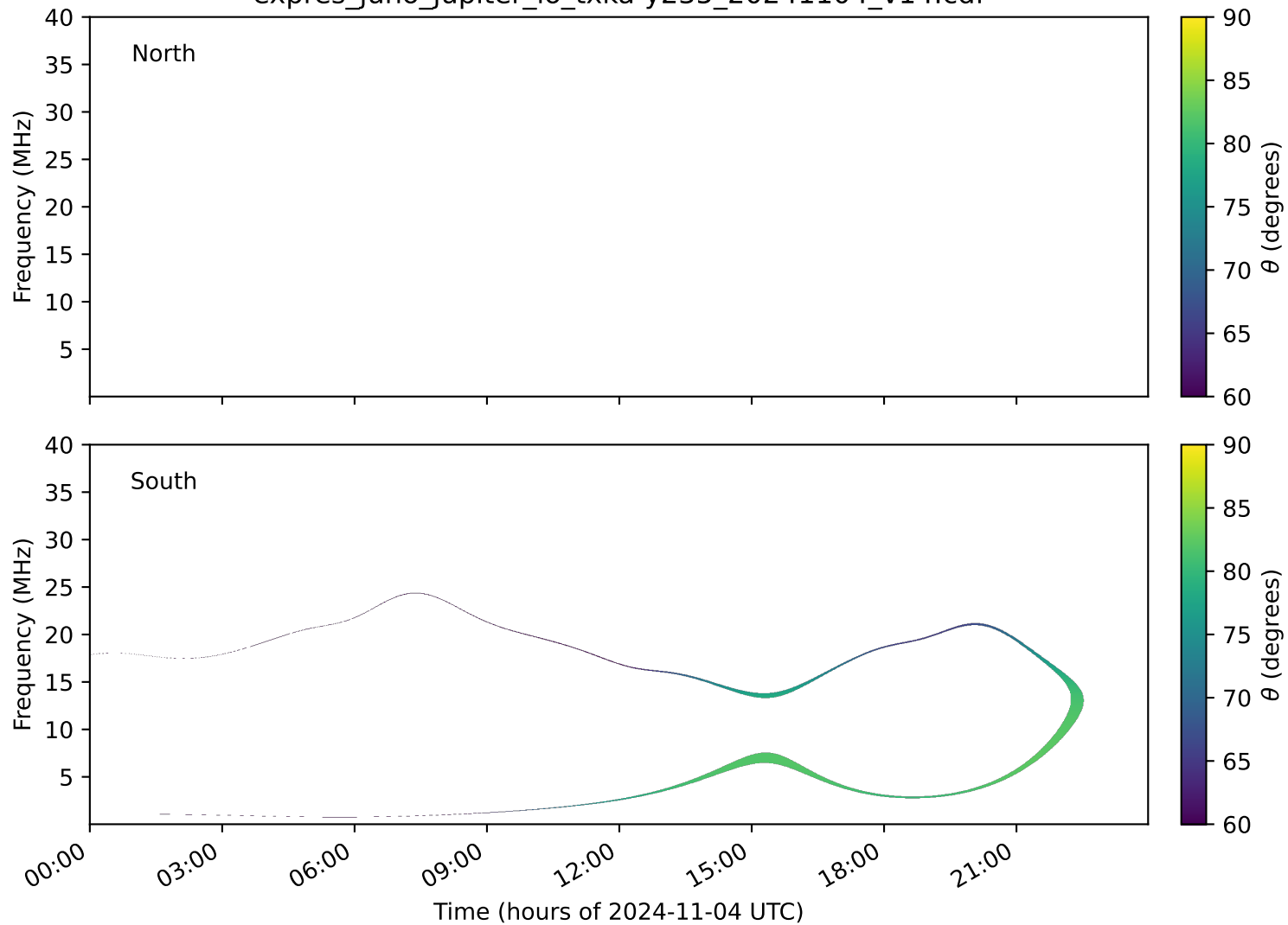
expres_juno_jupiter_io_txka-y235_20241104_v14.cdf
