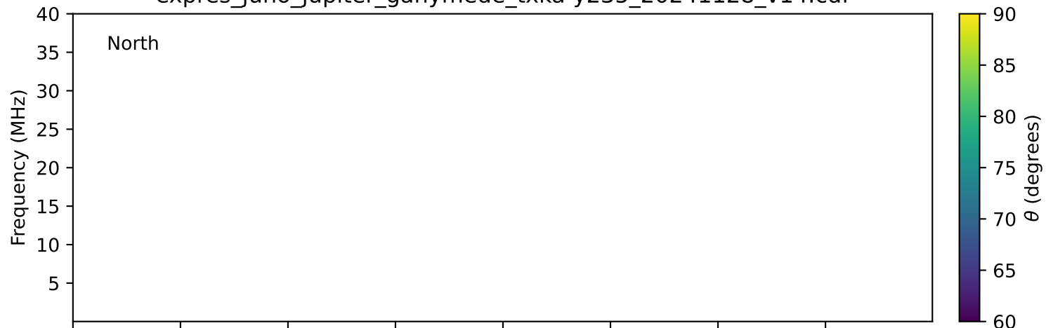
expres_juno_jupiter_ganymede_txka-y235_20241128_v14.cdf
