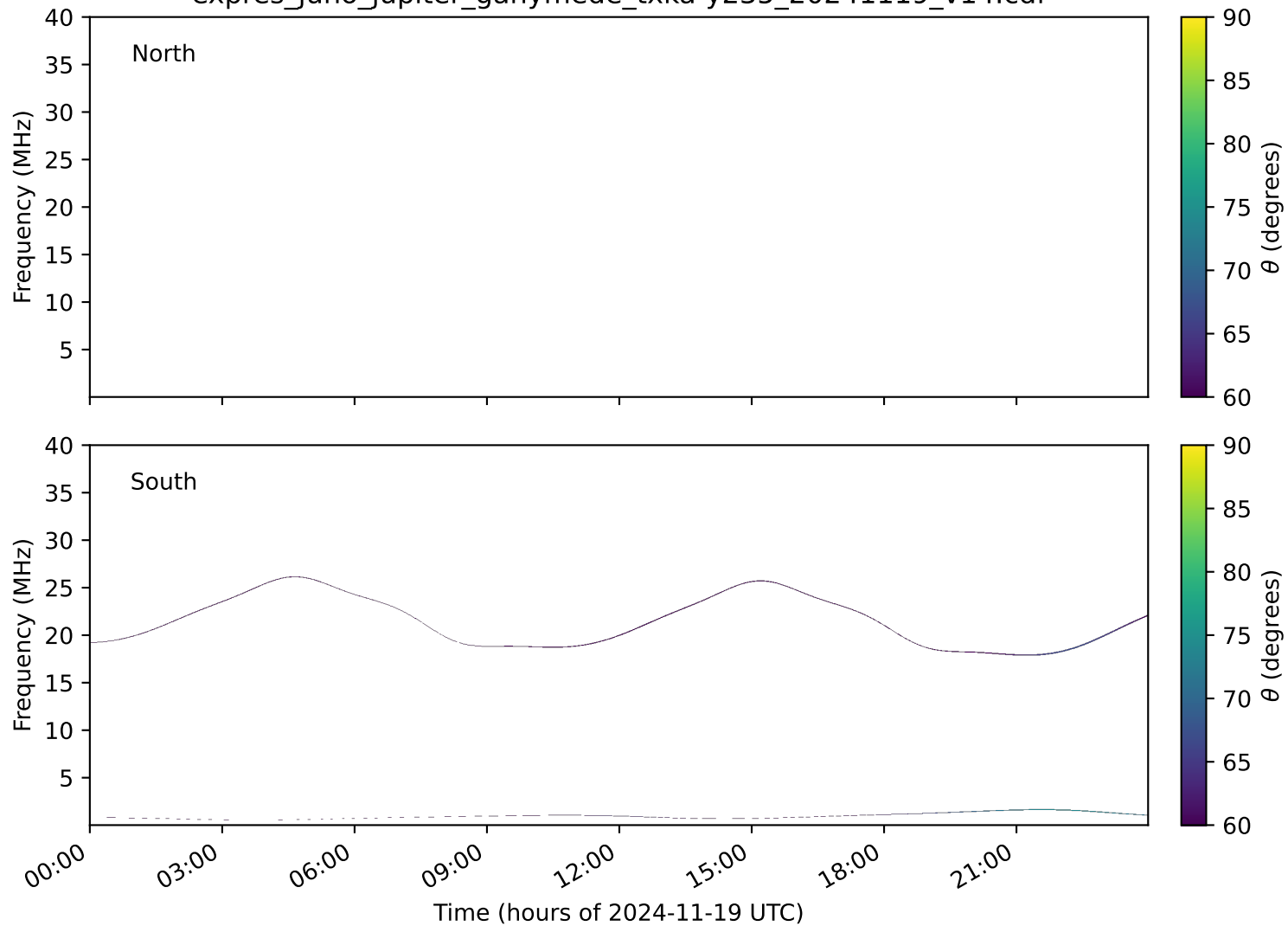
expres_juno_jupiter_ganymede_txka-y235_20241119_v14.cdf
