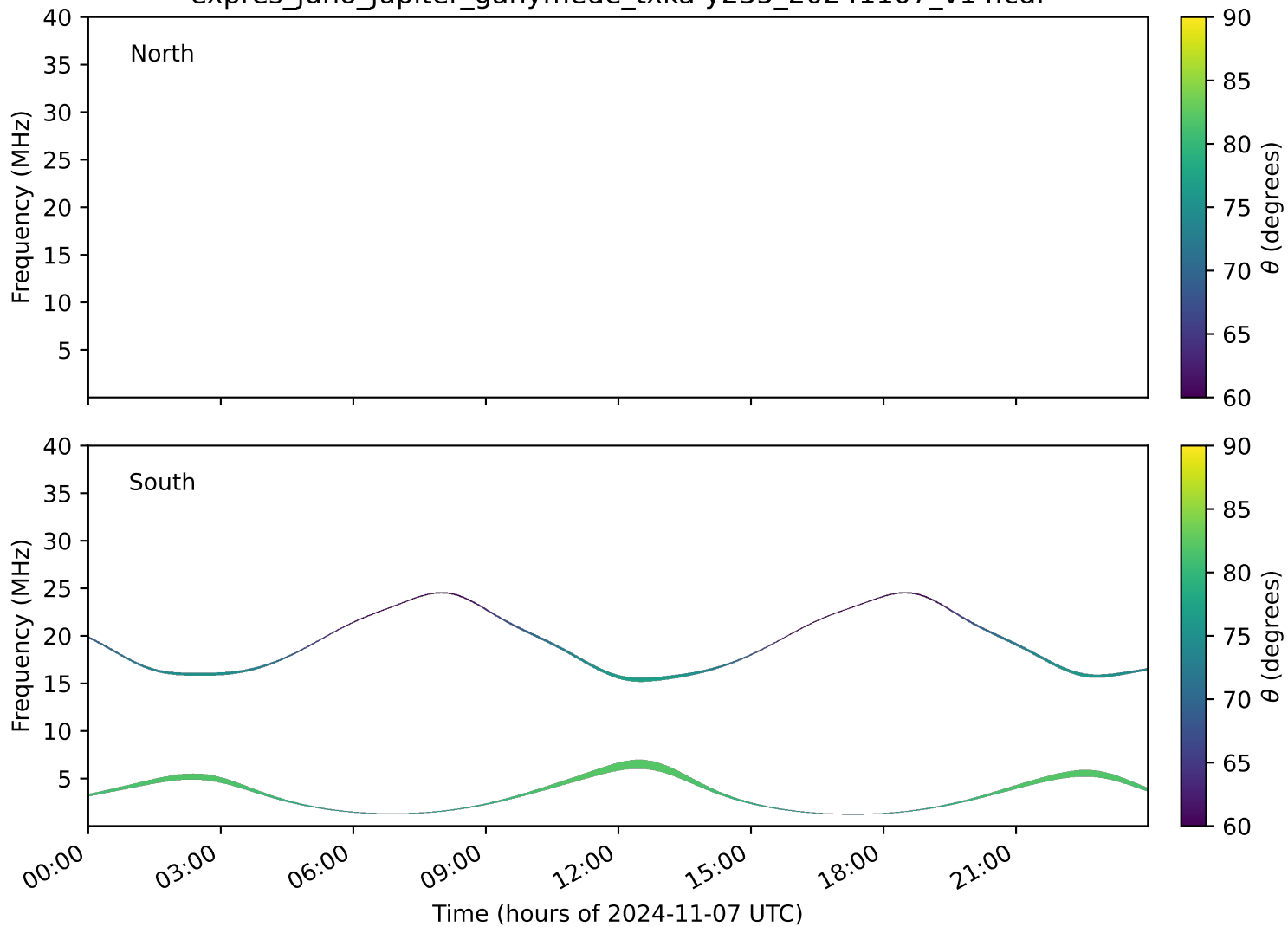
expres_juno_jupiter_ganymede_txka-y235_20241107_v14.cdf
