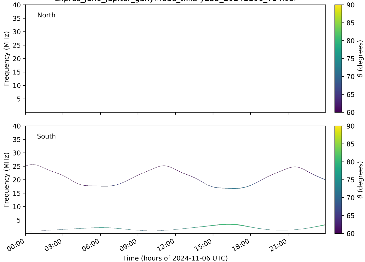
expres_juno_jupiter_ganymede_txka-y235_20241106_v14.cdf
