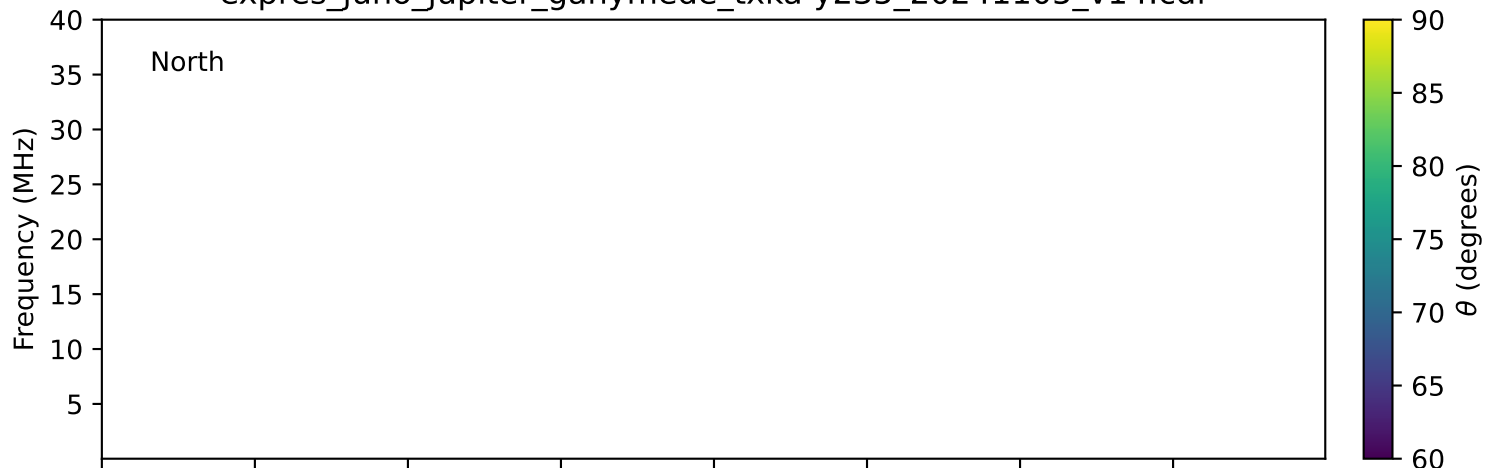
expres_juno_jupiter_ganymede_txka-y235_20241105_v14.cdf
