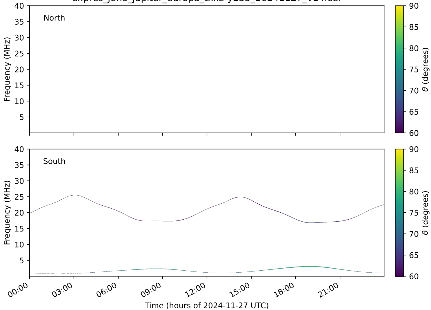
expres_juno_jupiter_europa_txka-y235_20241127_v14.cdf
