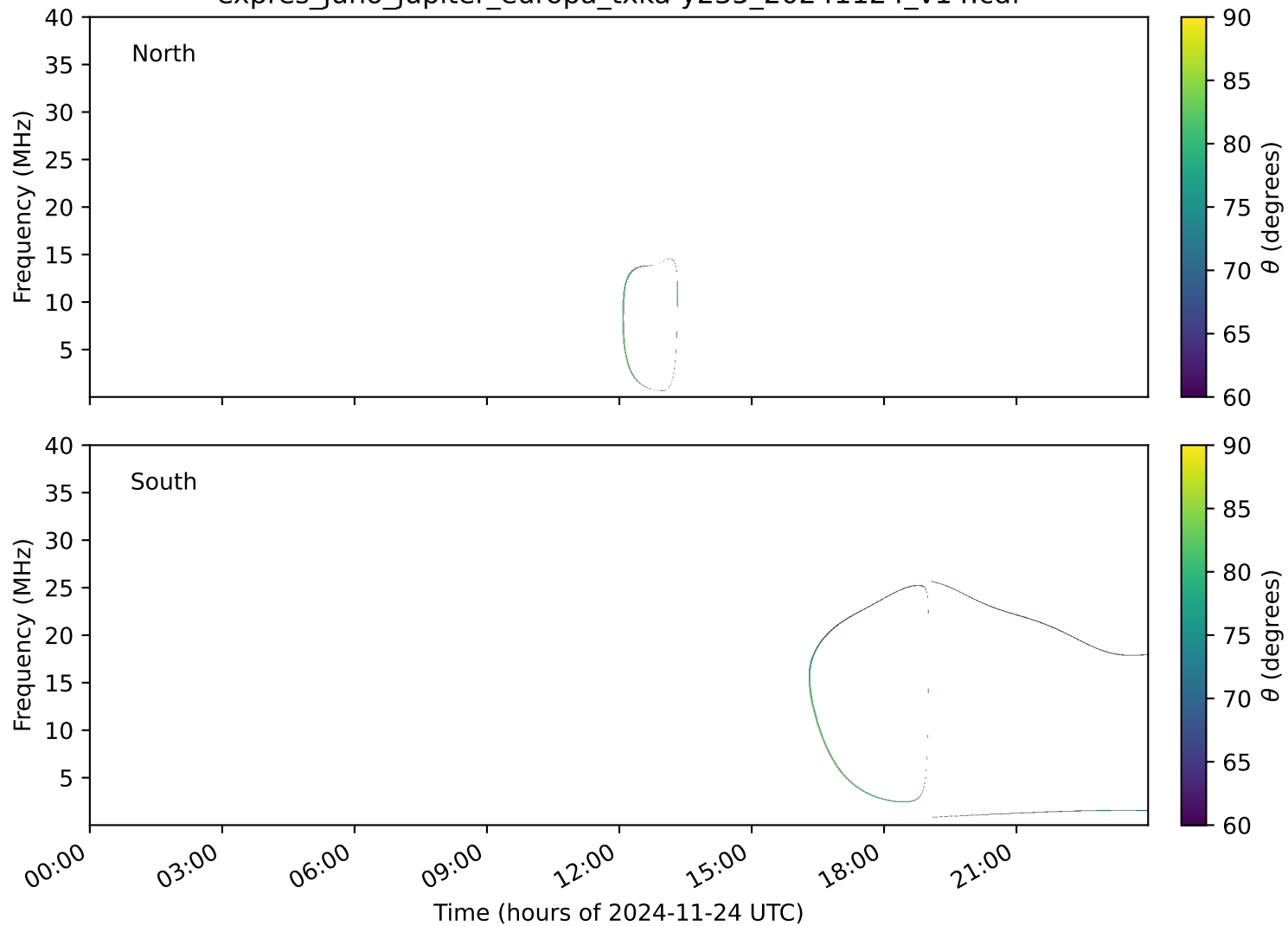
expres_juno_jupiter_europa_txka-y235_20241124_v14.cdf
