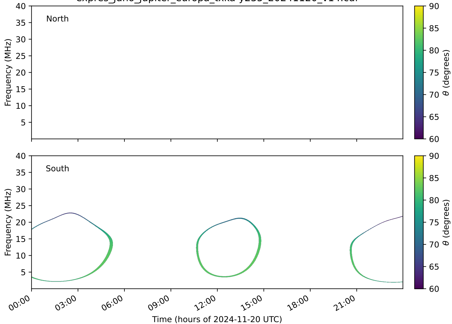
expres_juno_jupiter_europa_txka-y235_20241120_v14.cdf
