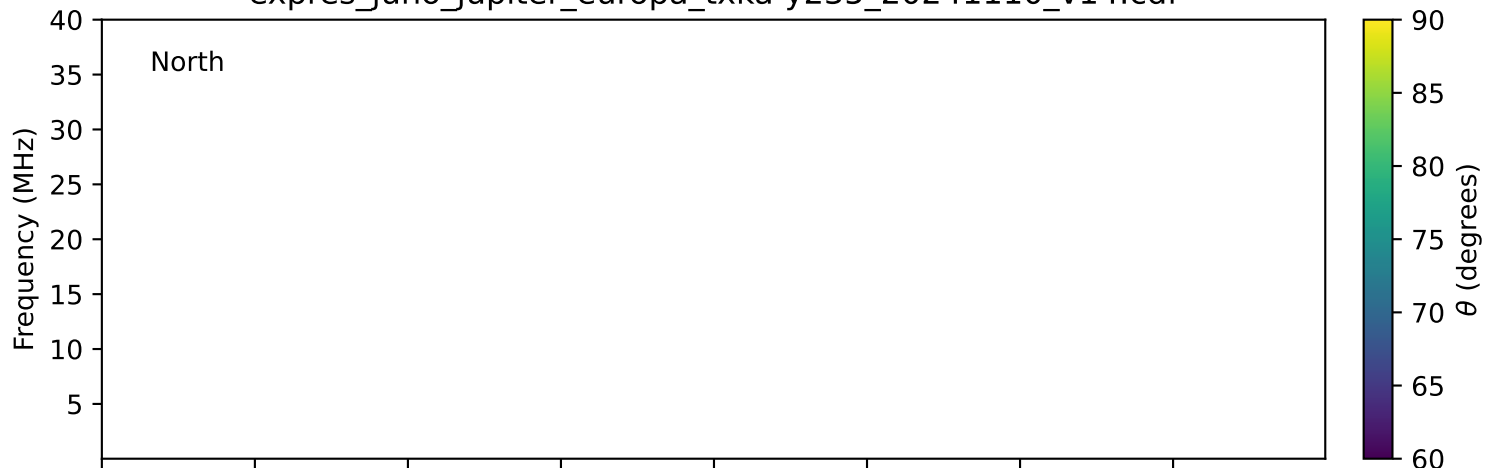
expres_juno_jupiter_europa_txka-y235_20241110_v14.cdf
