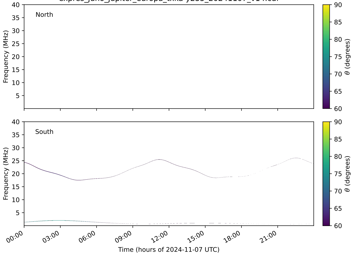
expres_juno_jupiter_europa_txka-y235_20241107_v14.cdf
