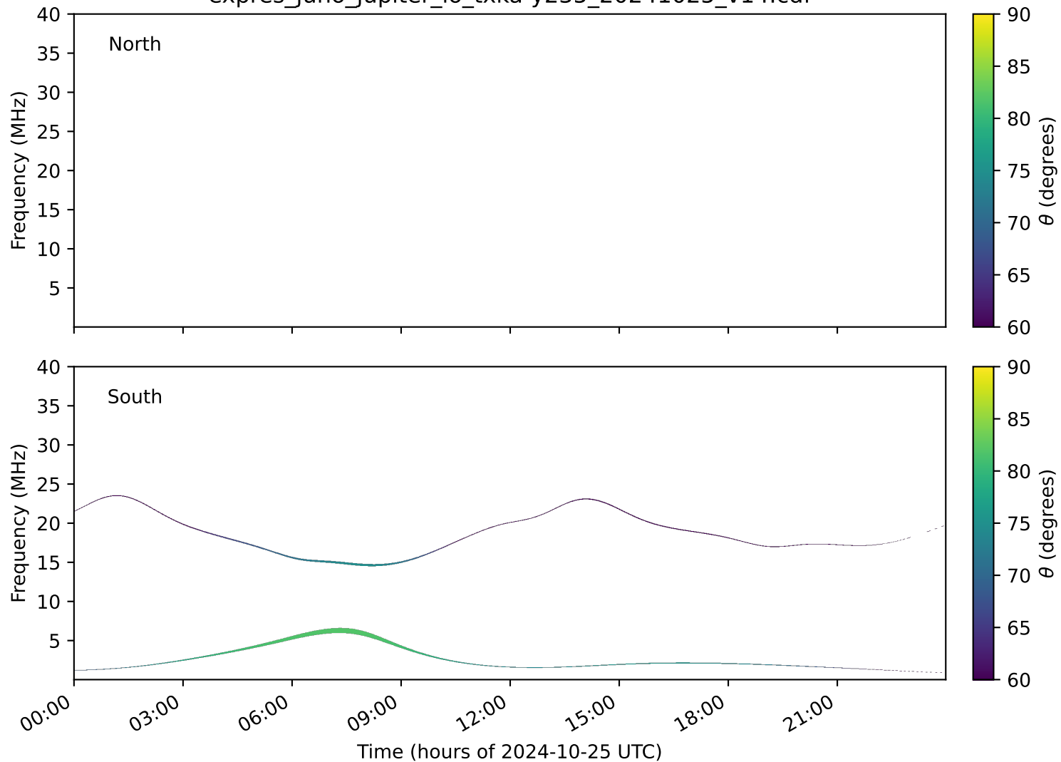
expres_juno_jupiter_io_txka-y235_20241025_v14.cdf
