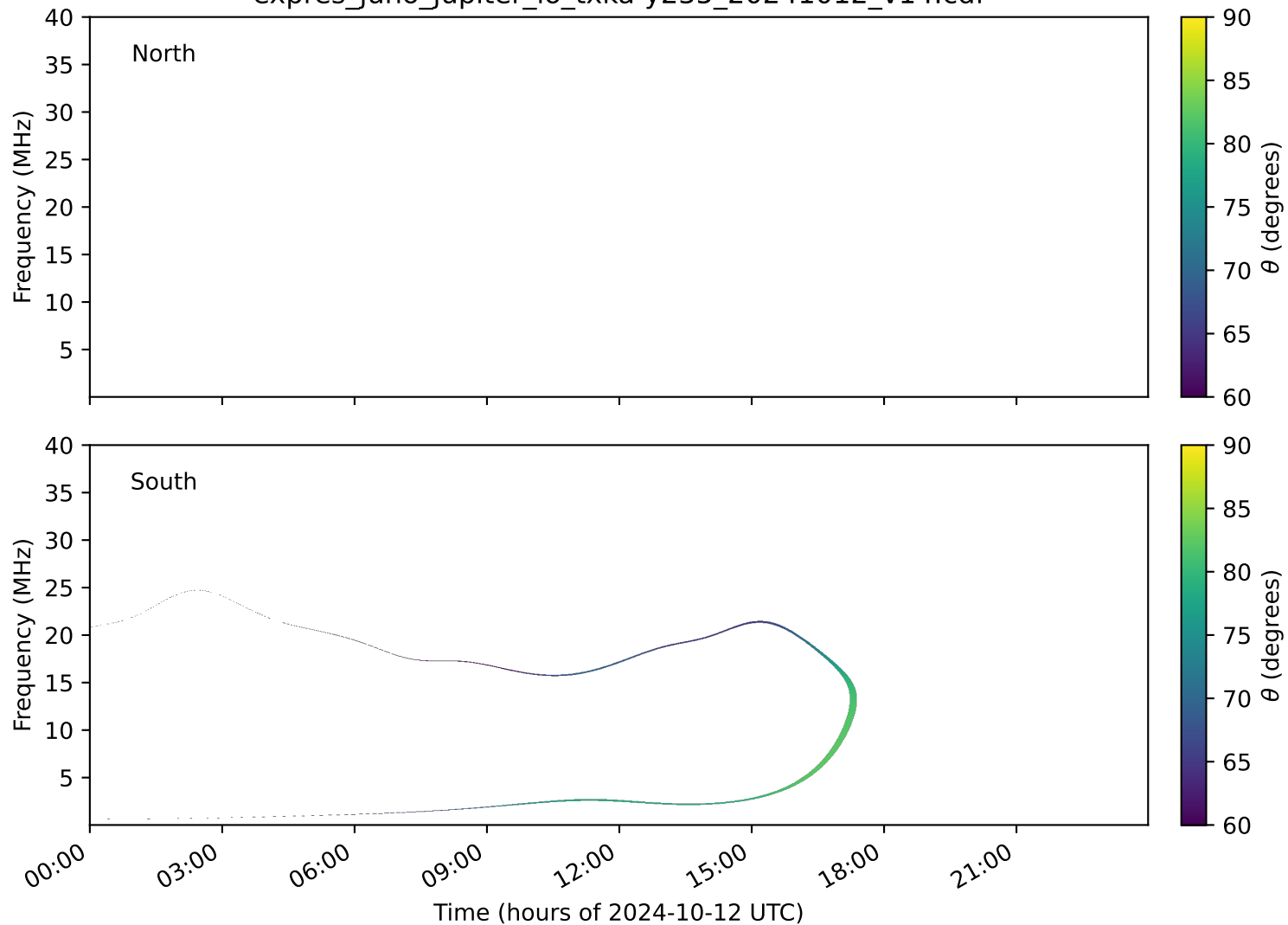
expres_juno_jupiter_io_txka-y235_20241012_v14.cdf
