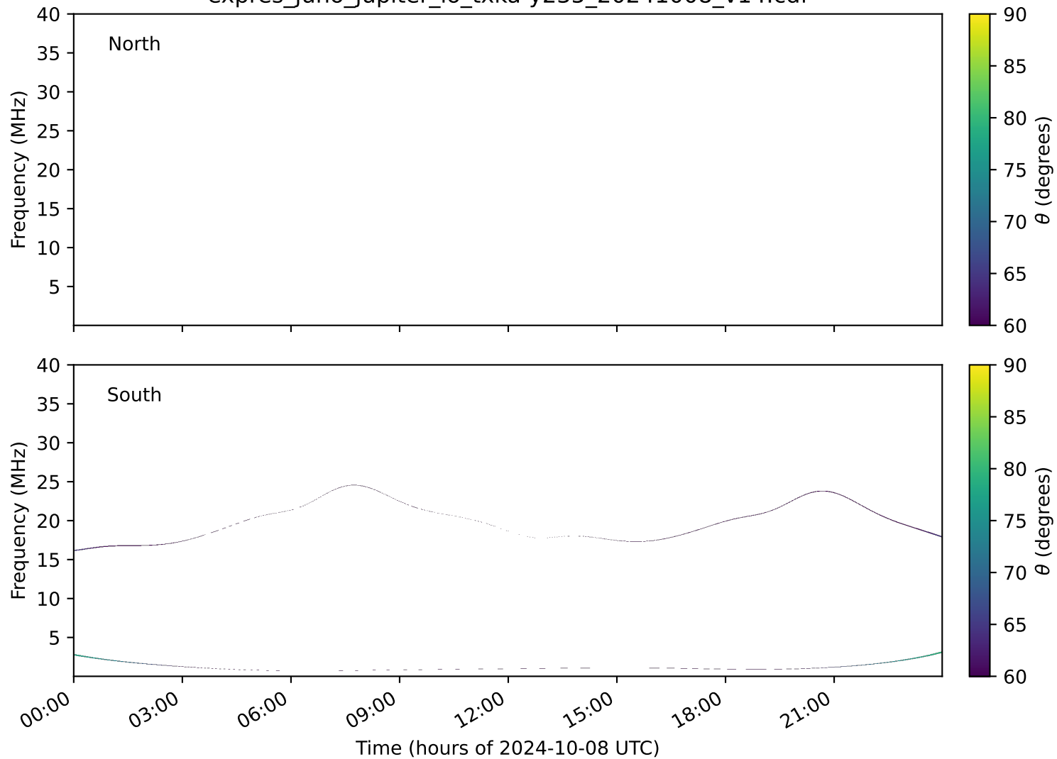
expres_juno_jupiter_io_txka-y235_20241008_v14.cdf
