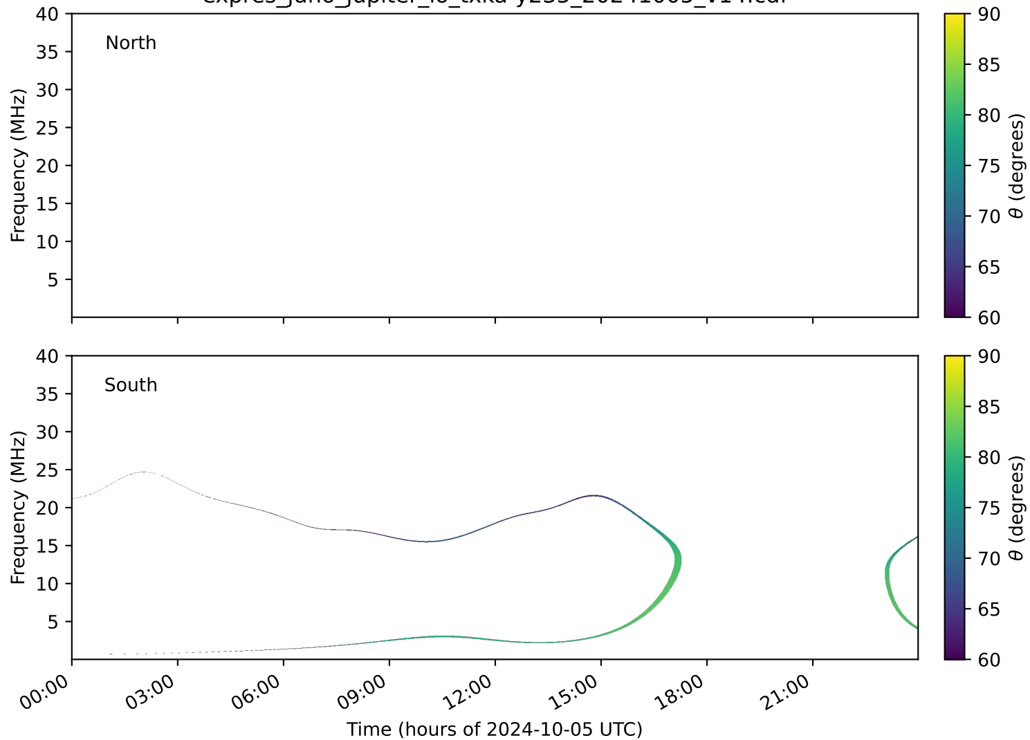
expres_juno_jupiter_io_txka-y235_20241005_v14.cdf
