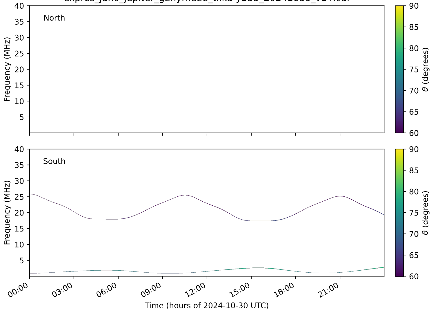
expres_juno_jupiter_ganymede_txka-y235_20241030_v14.cdf
