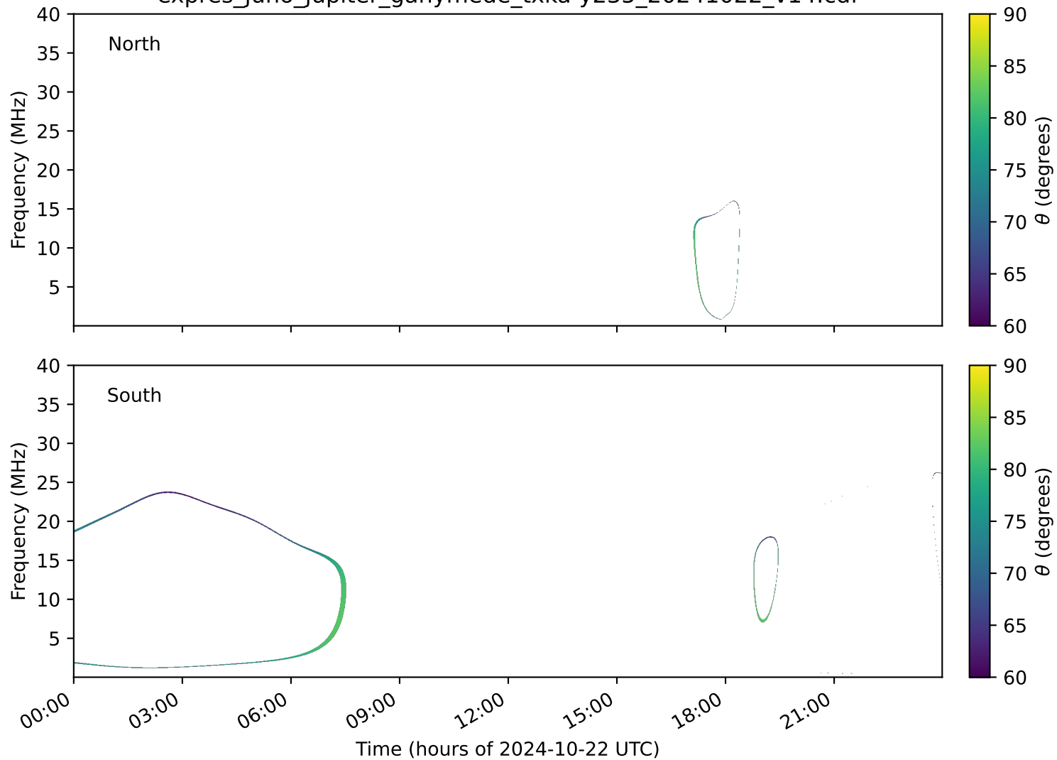
expres_juno_jupiter_ganymede_txka-y235_20241022_v14.cdf
