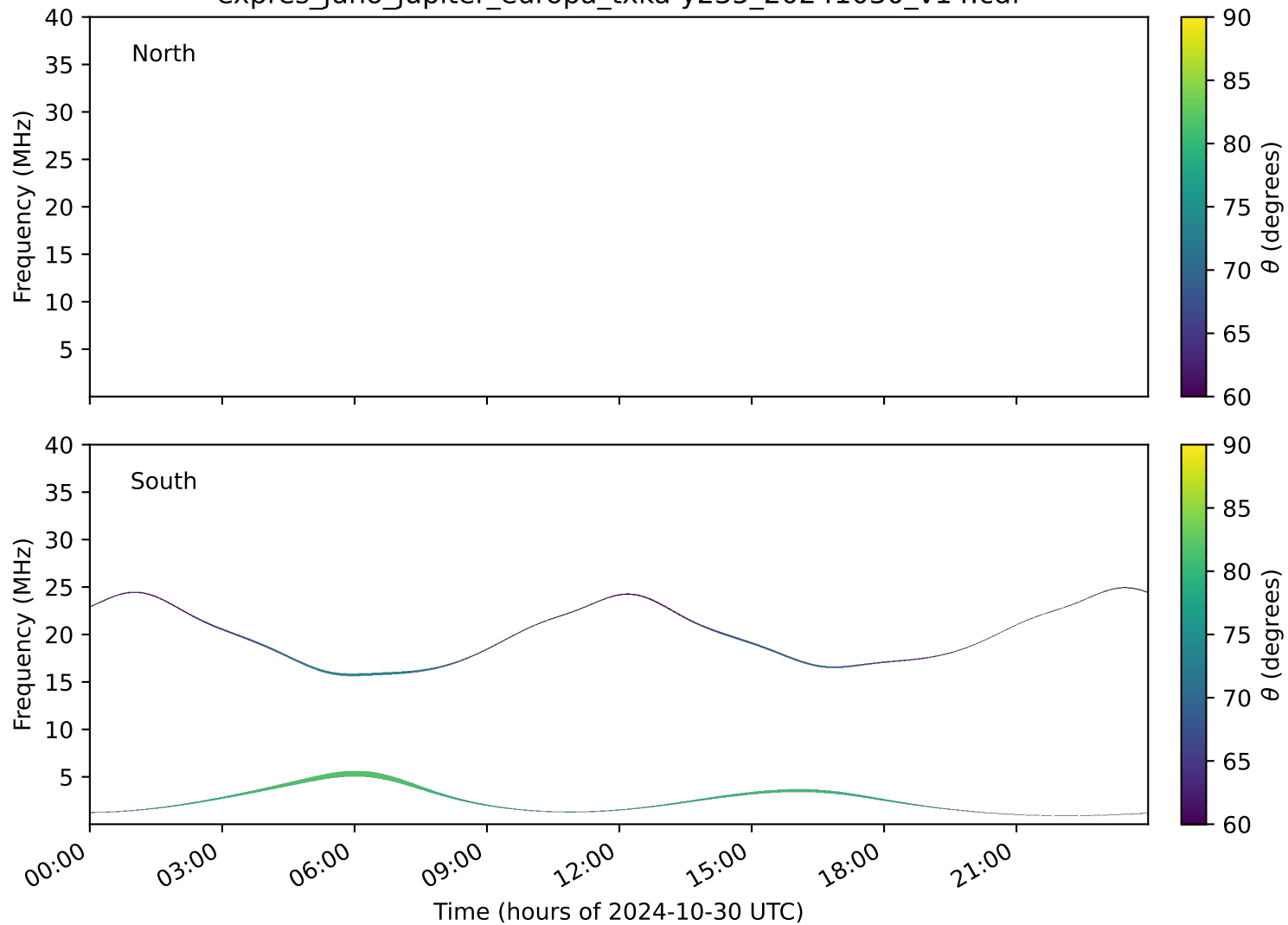
expres_juno_jupiter_europa_txka-y235_20241030_v14.cdf
