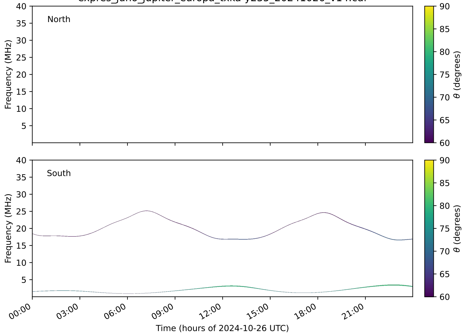
expres_juno_jupiter_europa_txka-y235_20241026_v14.cdf
