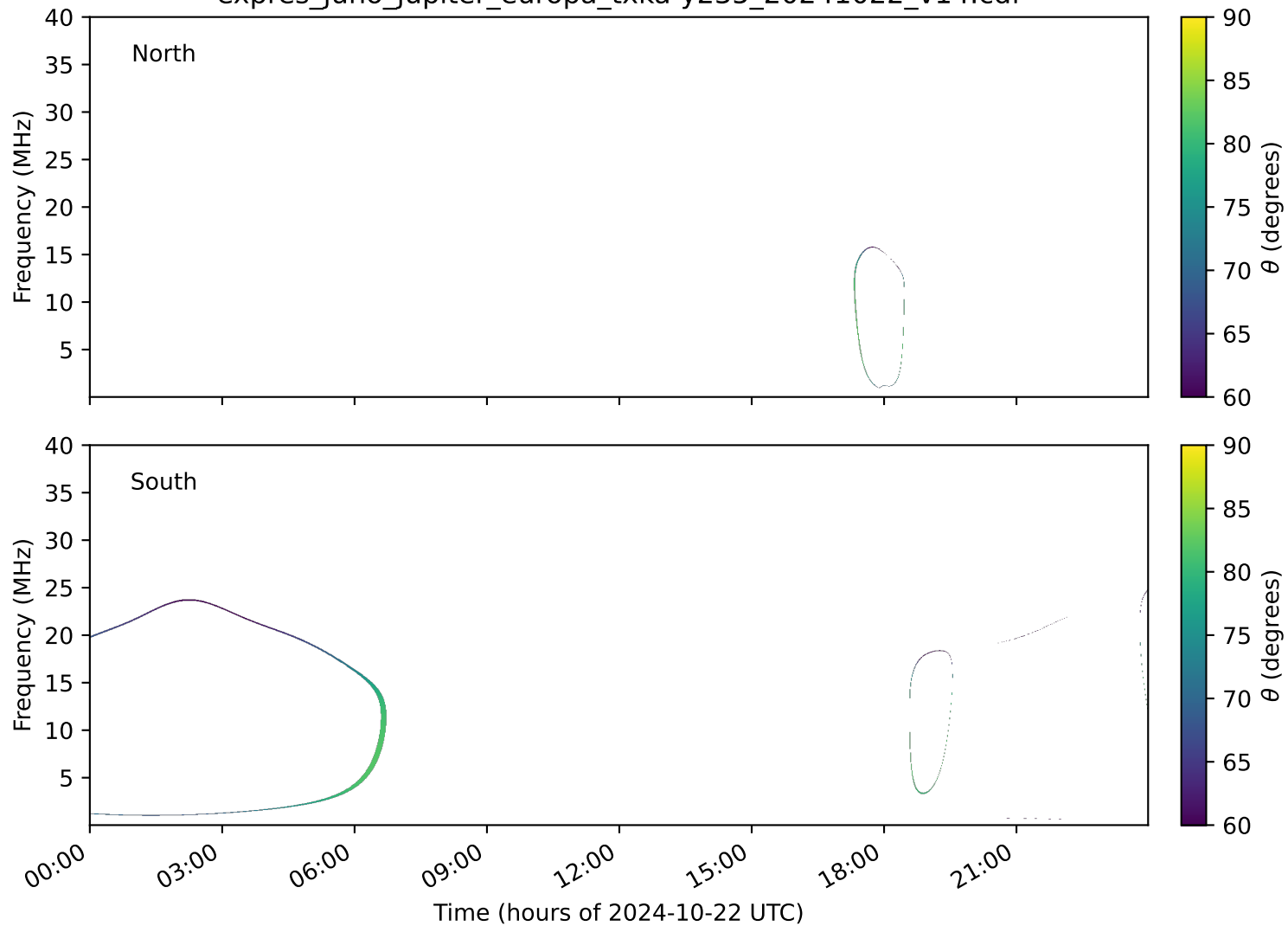
expres_juno_jupiter_europa_txka-y235_20241022_v14.cdf
