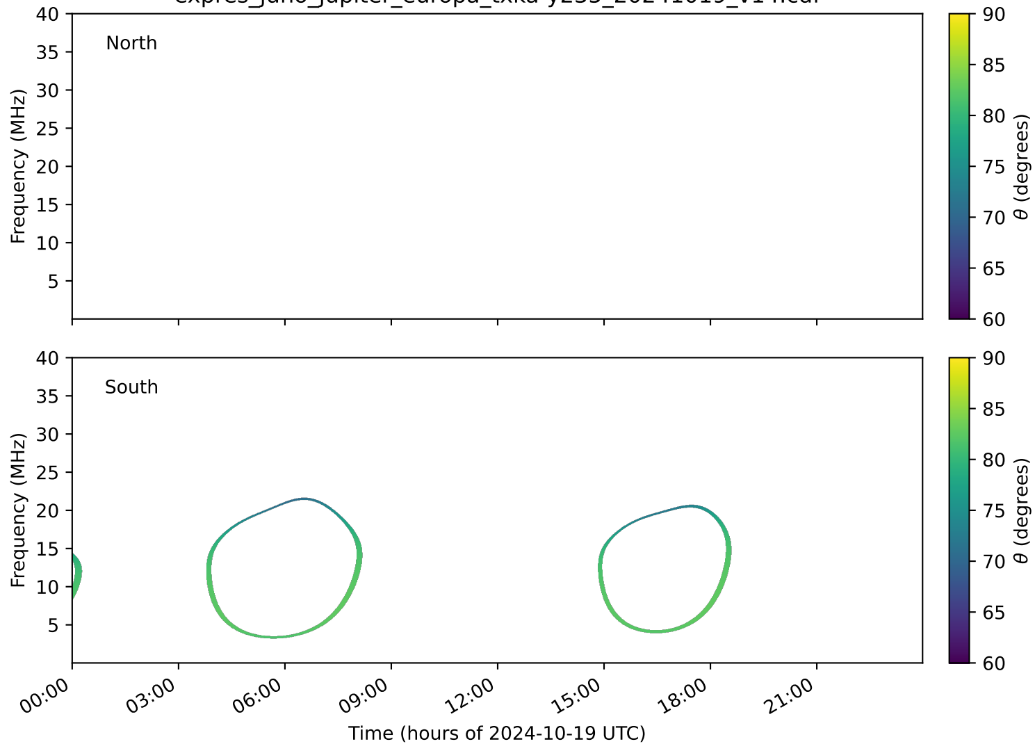
expres_juno_jupiter_europa_txka-y235_20241019_v14.cdf
