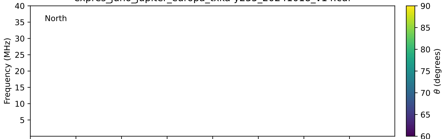
expres_juno_jupiter_europa_txka-y235_20241018_v14.cdf
