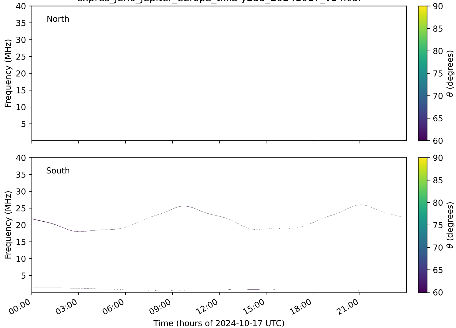
expres_juno_jupiter_europa_txka-y235_20241017_v14.cdf
