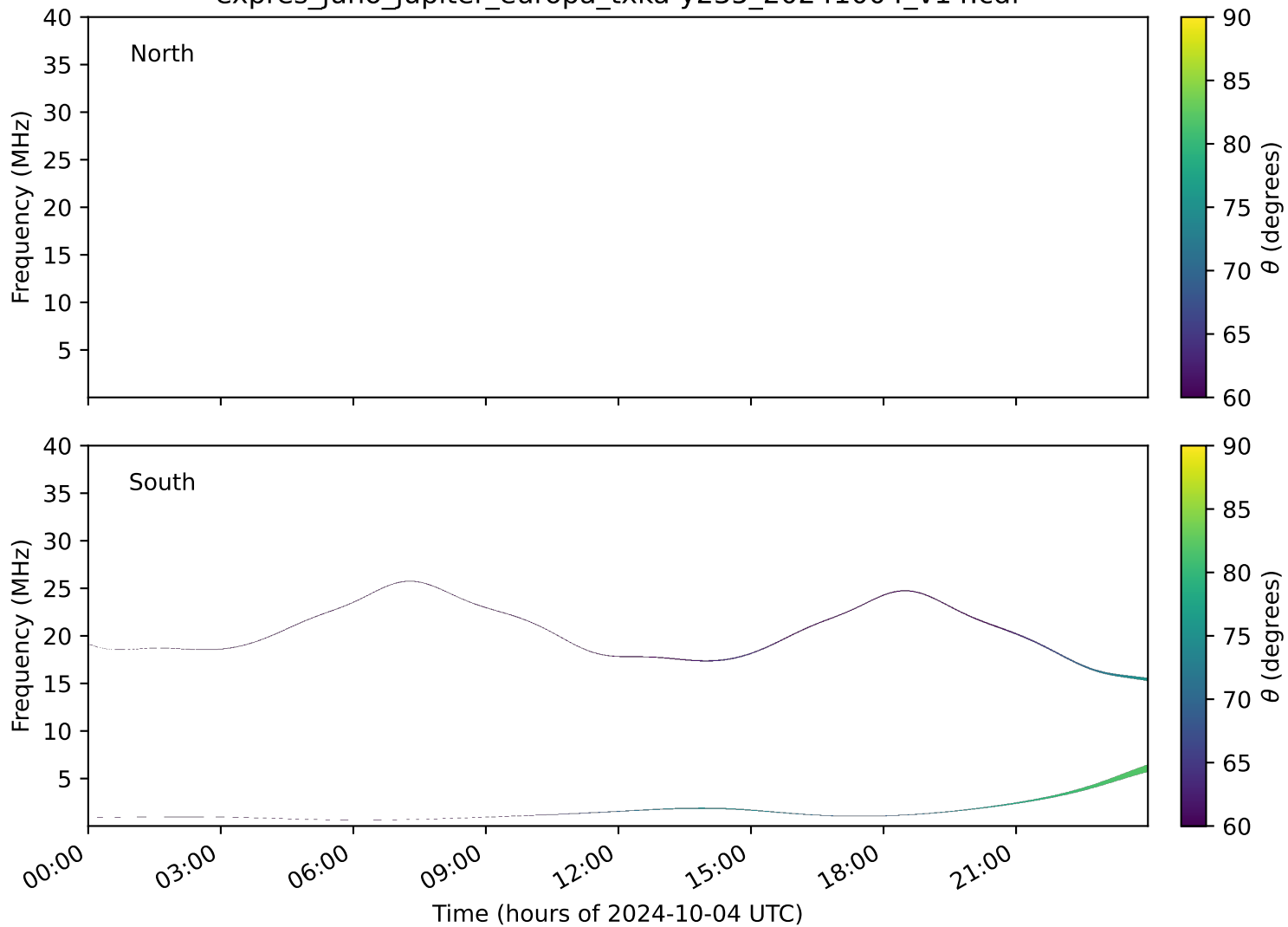
expres_juno_jupiter_europa_txka-y235_20241004_v14.cdf
