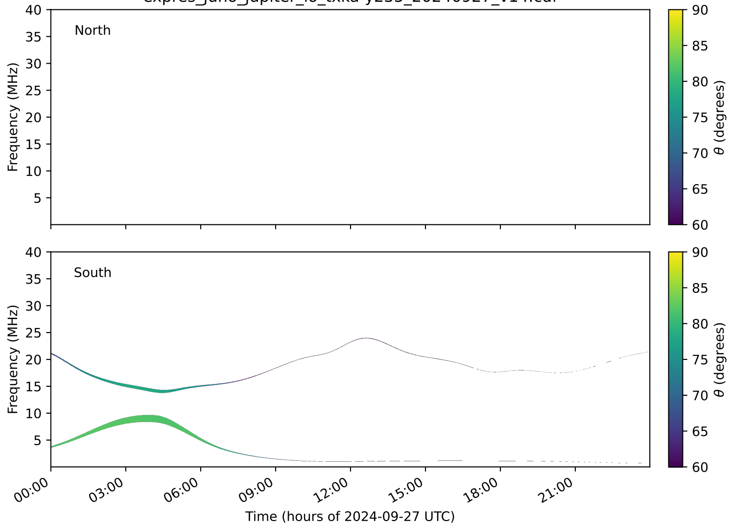
expres_juno_jupiter_io_txka-y235_20240927_v14.cdf
