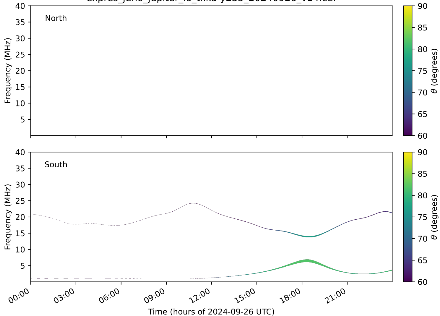
expres_juno_jupiter_io_txka-y235_20240926_v14.cdf
