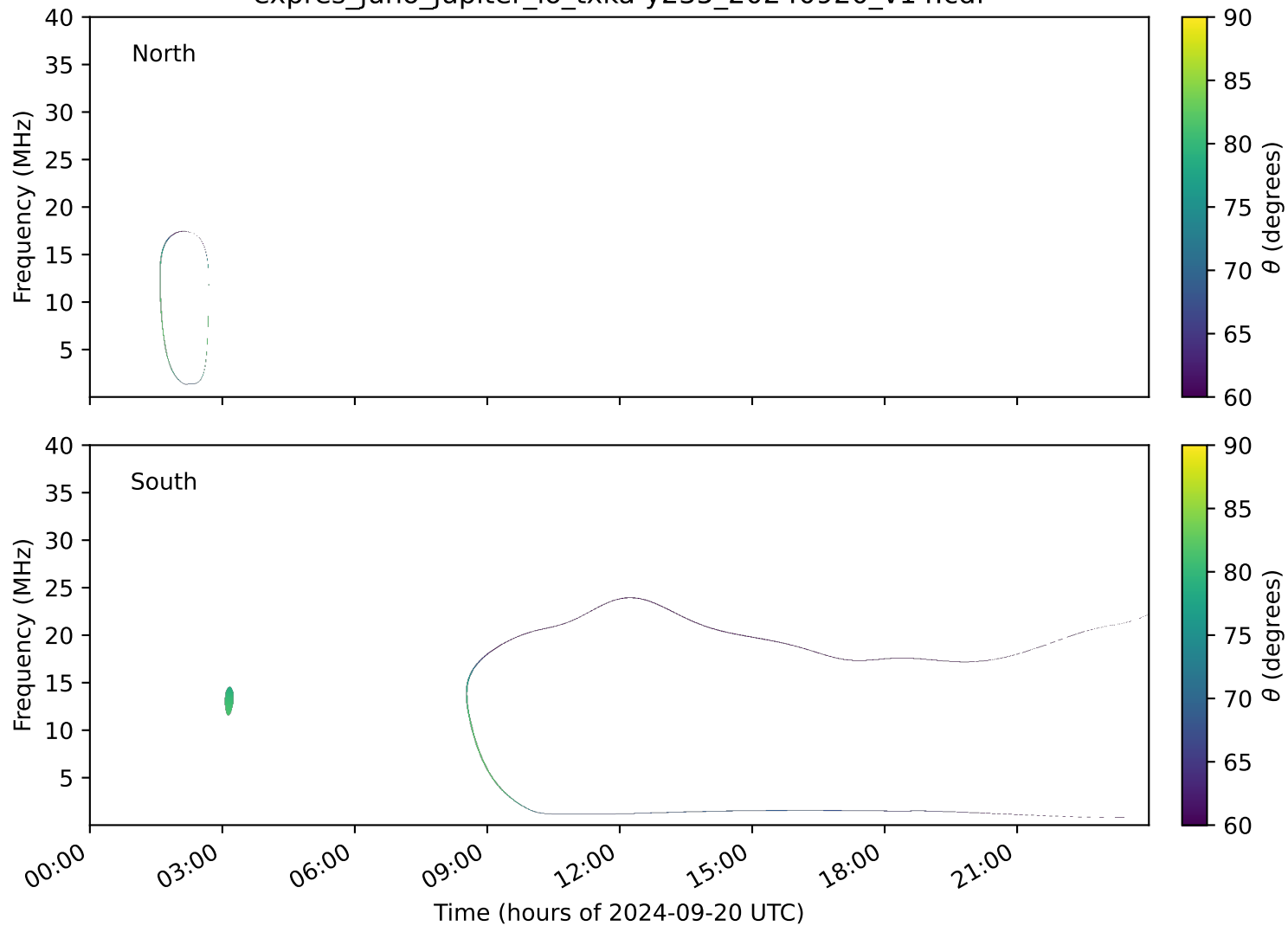
expres_juno_jupiter_io_txka-y235_20240920_v14.cdf
