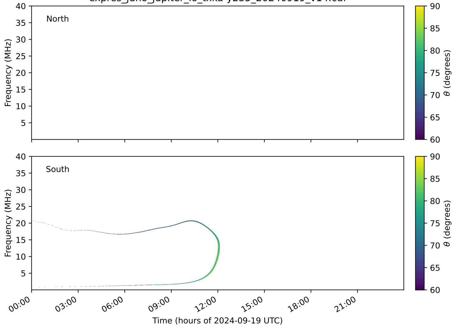
expres_juno_jupiter_io_txka-y235_20240919_v14.cdf
