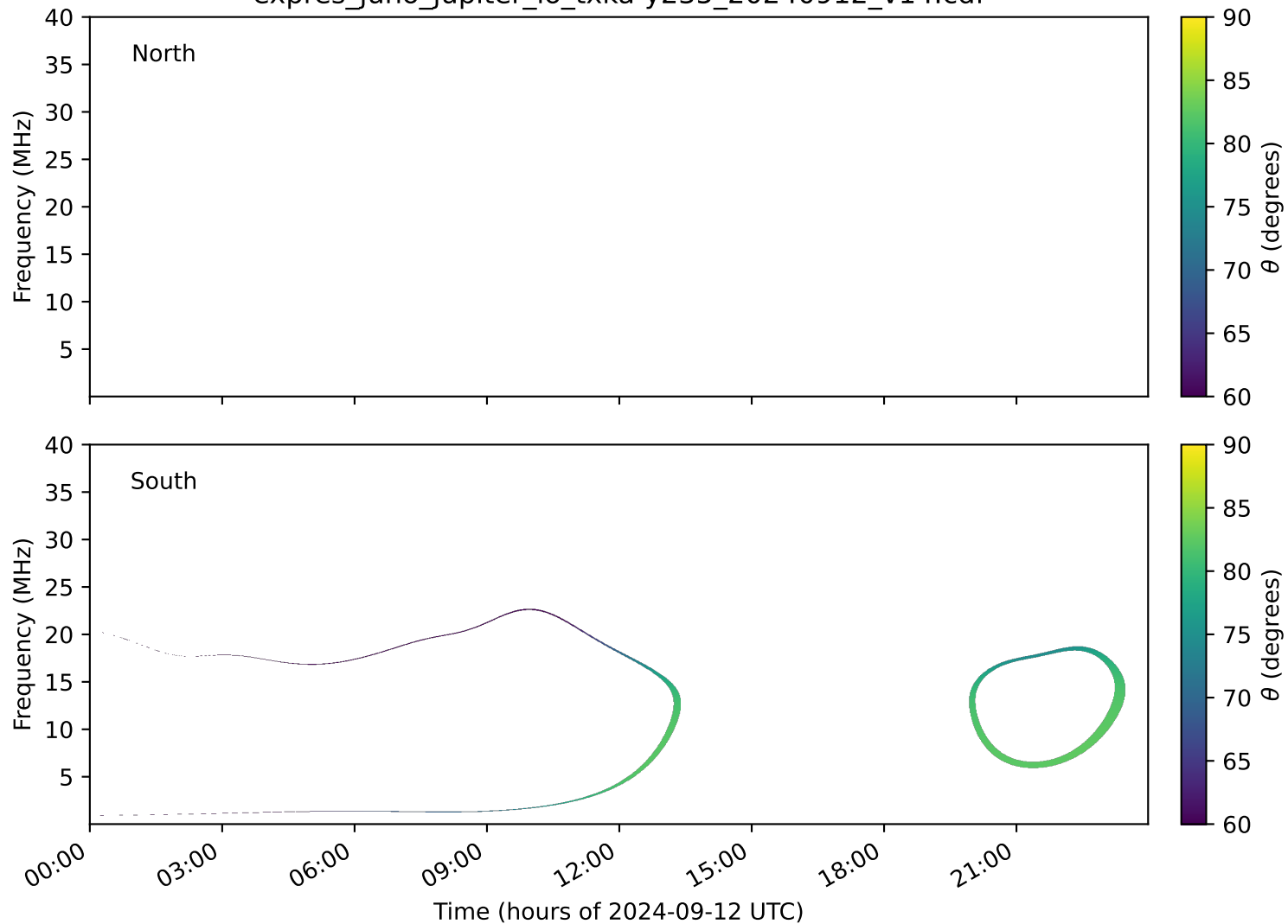
expres_juno_jupiter_io_txka-y235_20240912_v14.cdf
