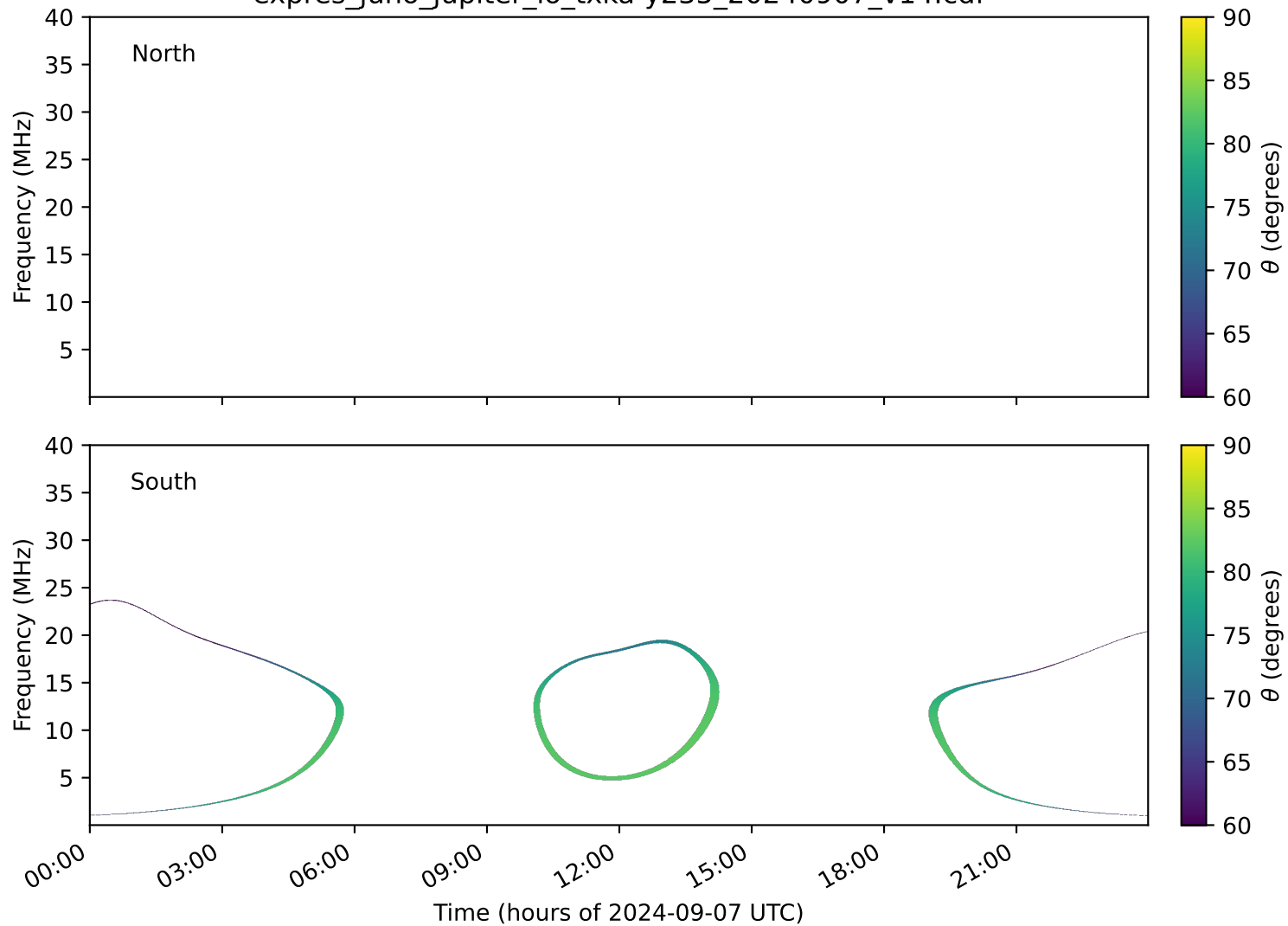
expres_juno_jupiter_io_txka-y235_20240907_v14.cdf
