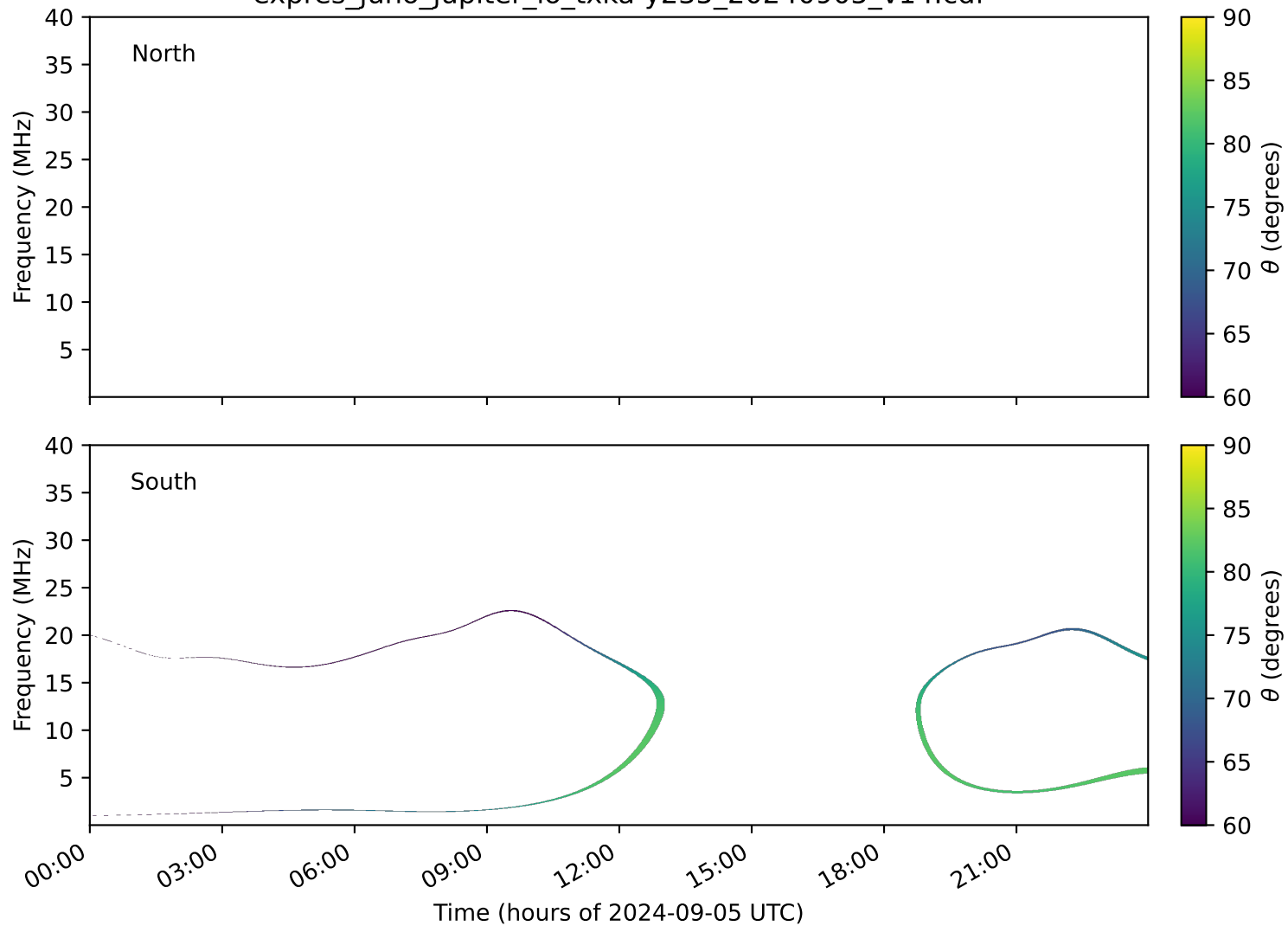
expres_juno_jupiter_io_txka-y235_20240905_v14.cdf
