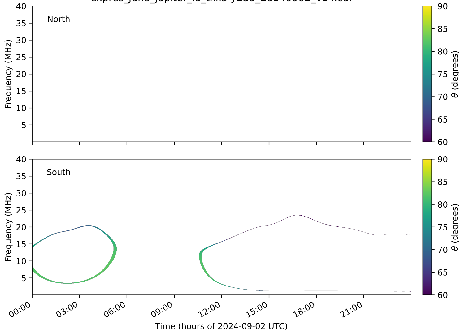
expres_juno_jupiter_io_txka-y235_20240902_v14.cdf
