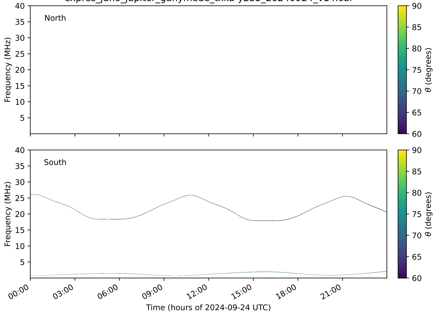
expres_juno_jupiter_ganymede_txka-y235_20240924_v14.cdf
