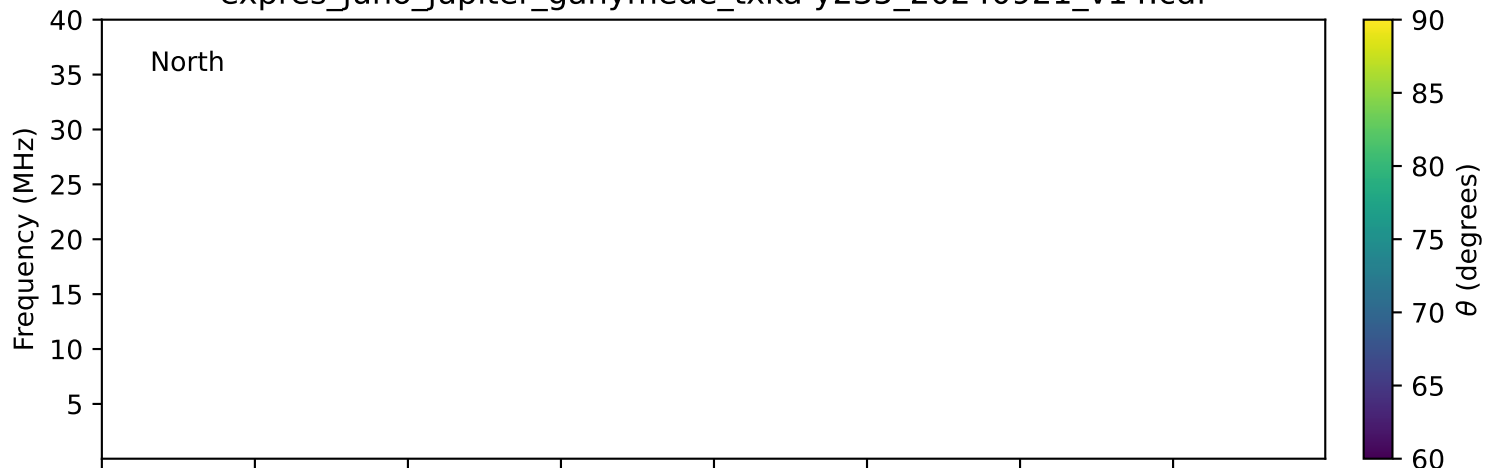
expres_juno_jupiter_ganymede_txka-y235_20240921_v14.cdf
