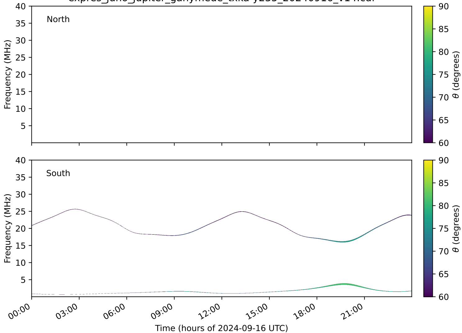
expres_juno_jupiter_ganymede_txka-y235_20240916_v14.cdf
