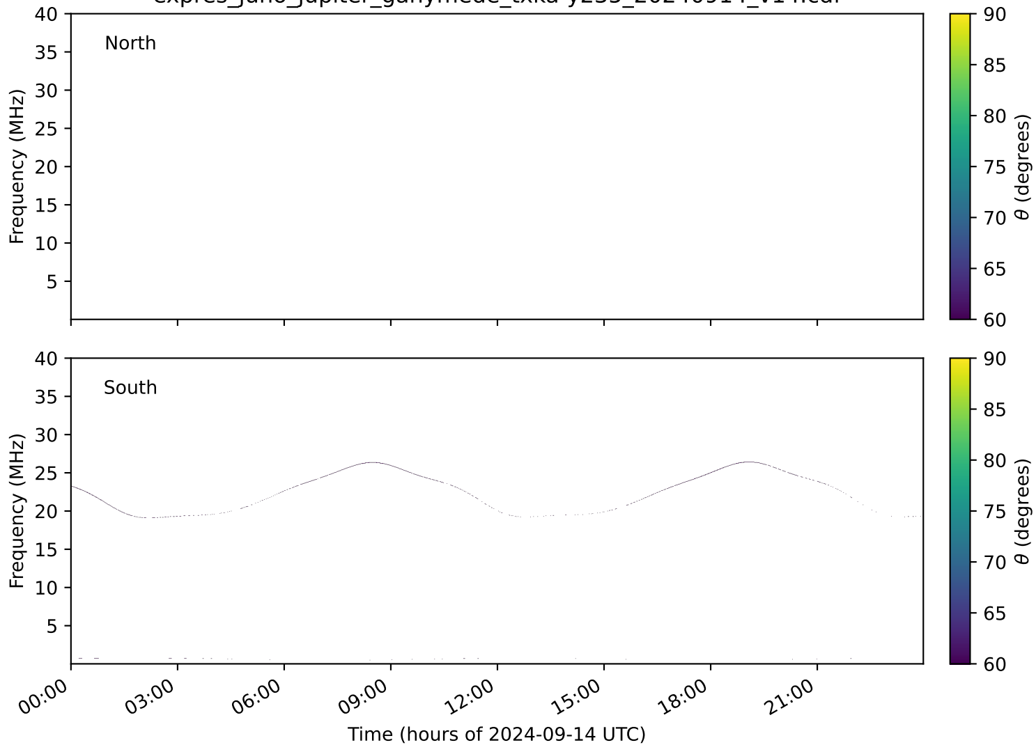
expres_juno_jupiter_ganymede_txka-y235_20240914_v14.cdf
