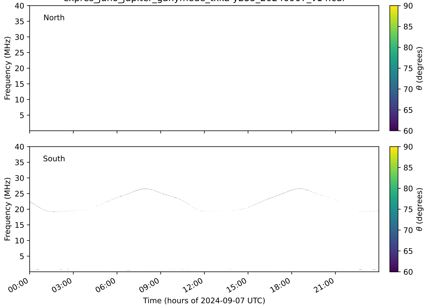
expres_juno_jupiter_ganymede_txka-y235_20240907_v14.cdf
