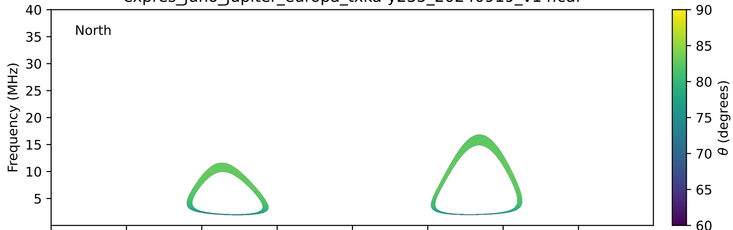
expres_juno_jupiter_europa_txka-y235_20240919_v14.cdf
