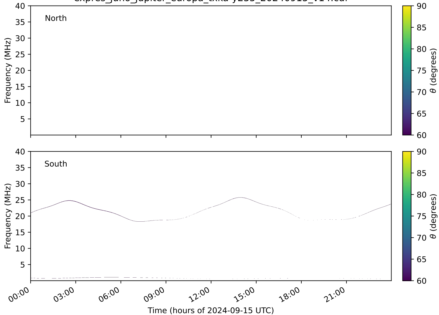
expres_juno_jupiter_europa_txka-y235_20240915_v14.cdf
