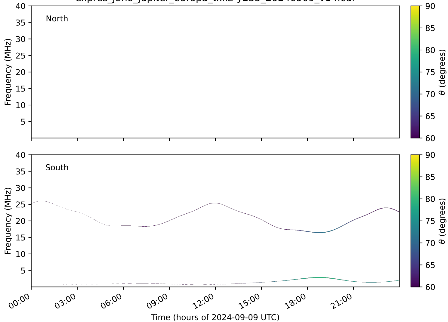
expres_juno_jupiter_europa_txka-y235_20240909_v14.cdf
